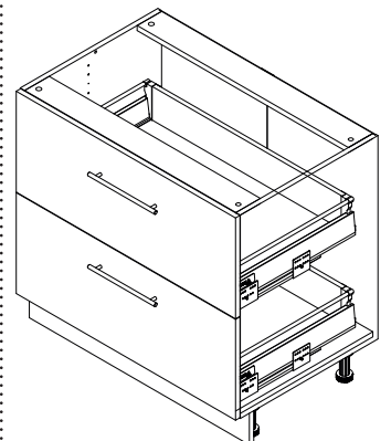
R-90-2MBOX LWH - 900x840x600
