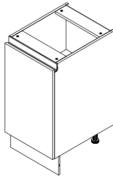
R-45-1K LHW-450X943X600
